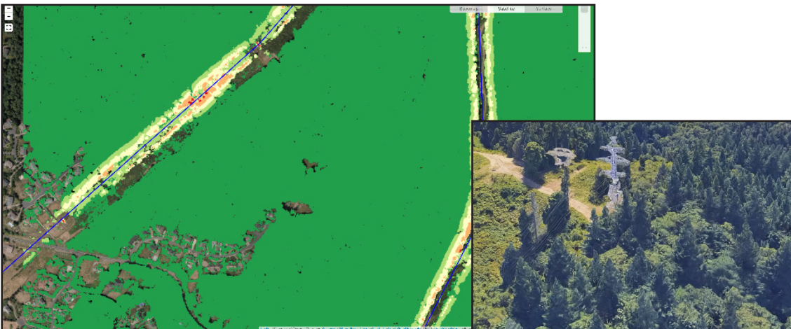
The risk of arcing is interpolated from Lidar data. 3D viewing provides context and verification.
